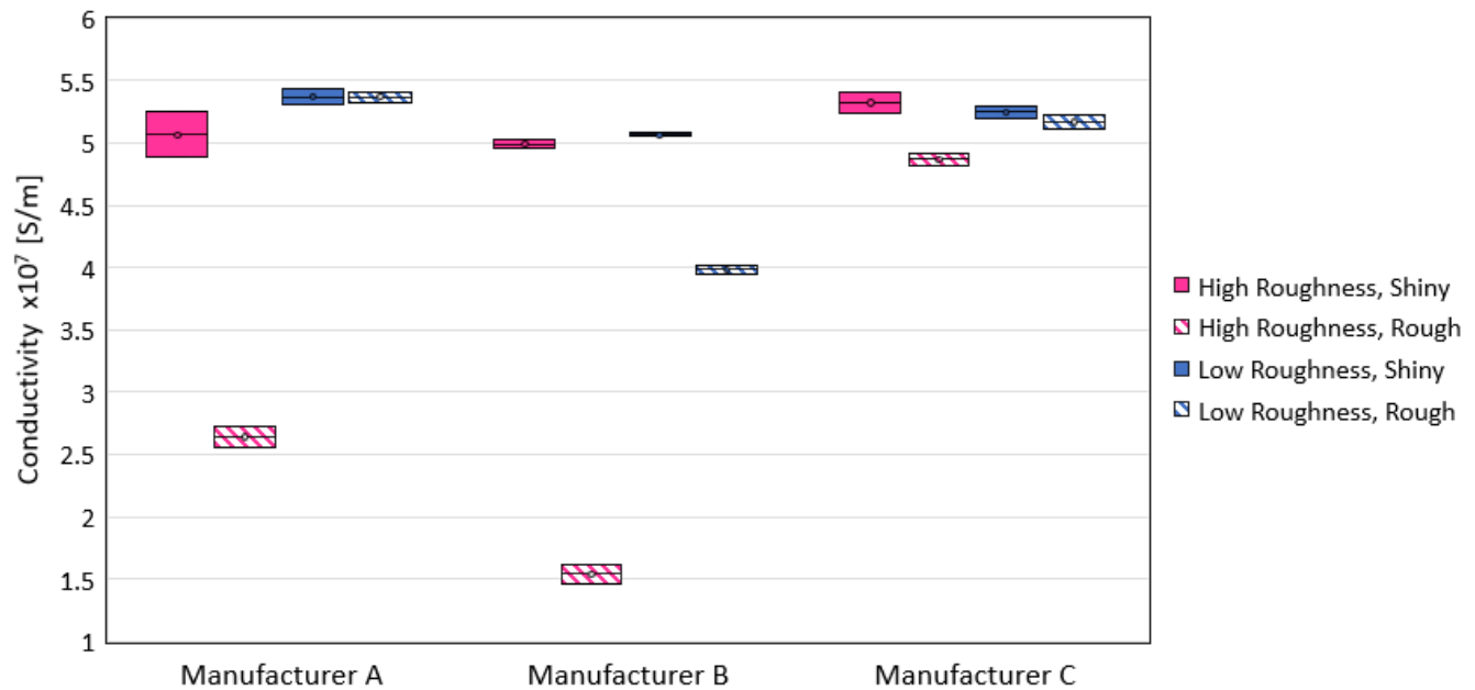
Figure 6. Effective conductivity of copper foil as seen from its two sides (denoted as Shiny and Rough), for two kinds of copper (Low Roughness and High Roughness), from three manufacturers (A,B,C), measured with SaDR at 13 GHz
