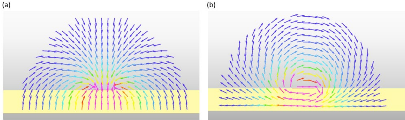
Figure 4. A 50 Ohm microstrip line and the (a) electric field and (b) magnetic field propagating through it.
