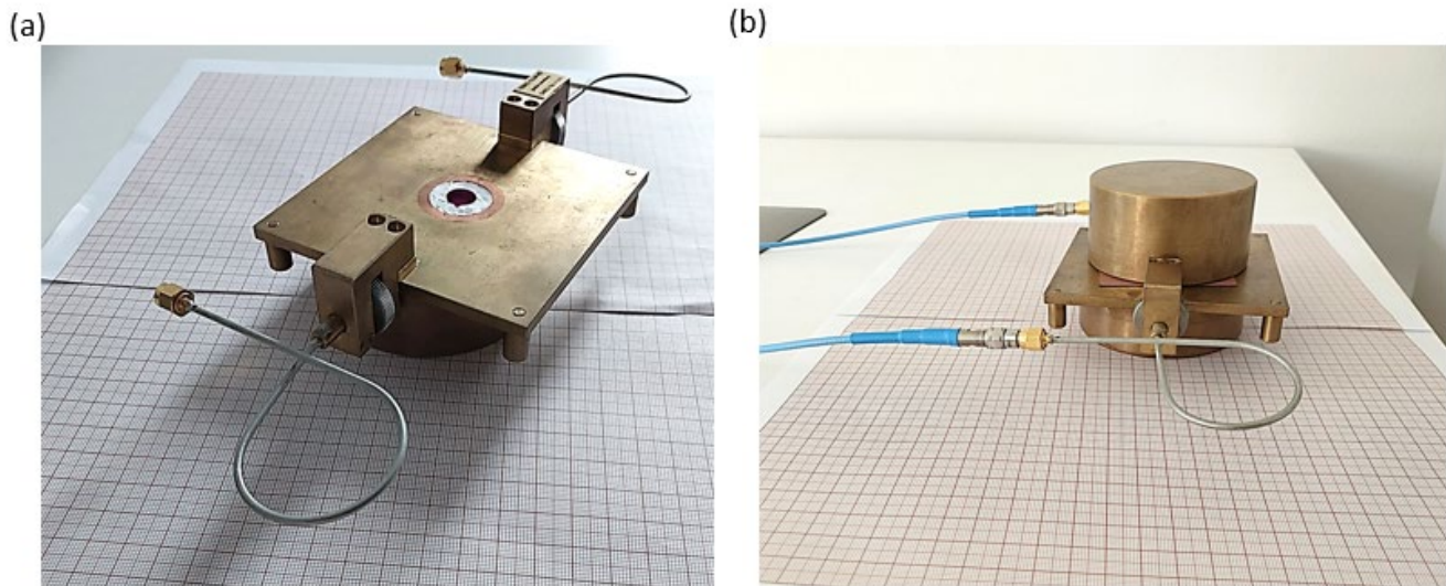
Figure 1. Sapphire Dielectric Resonator (a) without samples and (b) with samples pressed down with metal cylinders.
