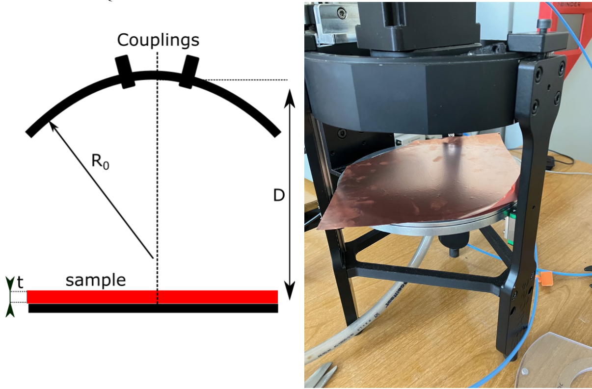
Figure 2. (a) Schematic with marking of dimensions necessary for extraction of material parameters and (b) actual pc-FPOR measurement set-up with MUT
