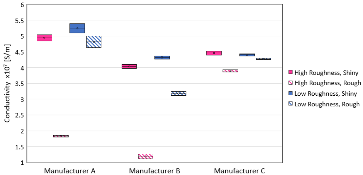
Figure 7. Effective conductivity of copper foil as seen from its two sides (denoted as Shiny and Rough), for two kinds of copper (Low Roughness and High Roughness), from three manufacturers (A,B,C), measured with SaDR at 21 GHz.
