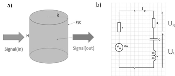
Figure 3. Theoretical model of a) cylindrical resonator and its b) equivalent circuit for one selected resonance.
